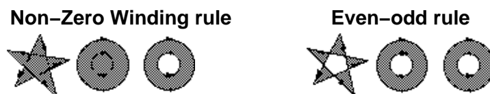
Figure 7: Fill Rules
