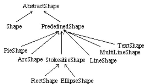
Figure 15: Predefined Shape Inheritance Hierarchy
