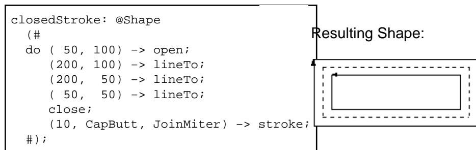
Figure 9: The stroke operation applied to a closed shape
