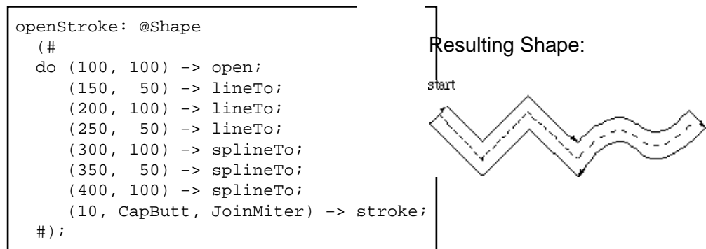
Figure 8: Stroke operation applied to an open shape
