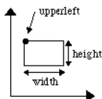
Figure 4: Coordinate System
