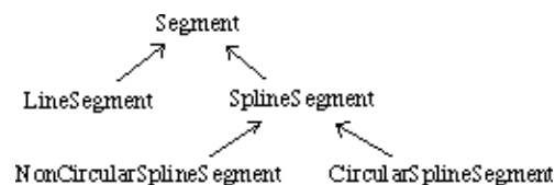
Figure 5: The segment hierarchy
